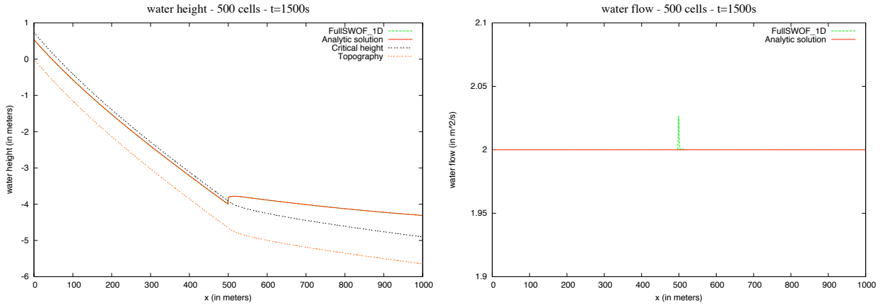
Figure 7: Torrential/fluviol Mac Donald like test with Darcy-Weisbach friction coefficient
